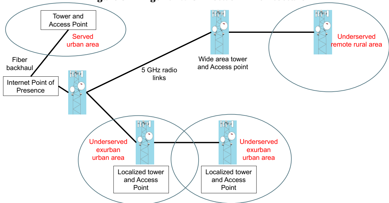
Figure 3-1. Nigeria: WISP Network Architecture
